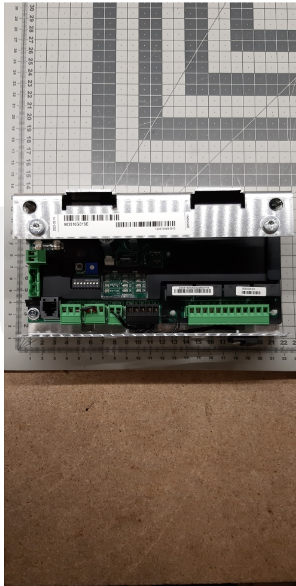
903510G01SE ECO CF EN81-20/50 H+/AE Controller
