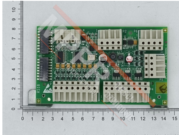
RS18 remote station PCB with horizontal connectors.
