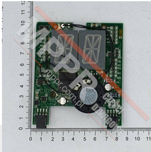
FAA23600AB1 Hall position indicator 15 PCB for OTIS 2000
