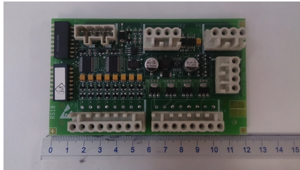
RS18 remote station PCB with vertical connectors.
